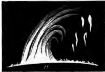
CHANGED APPEARANCE OF THE SOLAR 'THUNDER CLOUD.'
